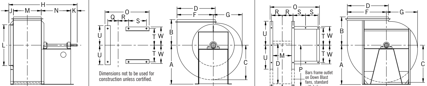
DIMENSIONS [INCHES]
